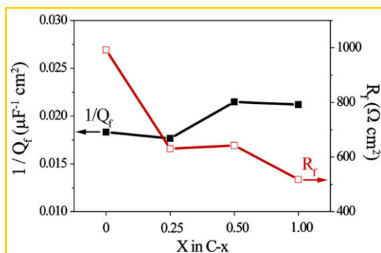
Fig. 7. Impedance and relative thickness ( 1/Q_r ) of oxide layer vs. Al content x plots.
