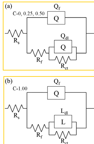
Fig. 6. EIS equivalent circuits (a) for alloys C-0, C-0.25, and C-0.50, and (b) for alloy C-1.00.
